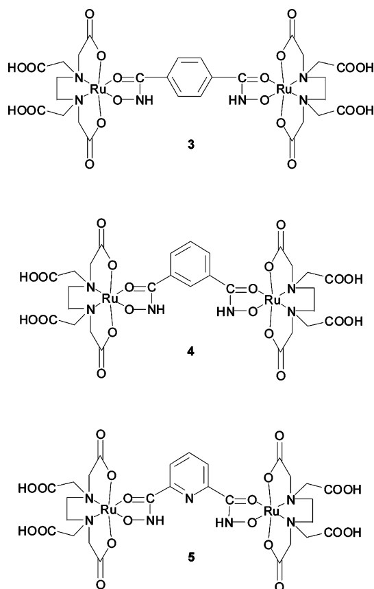
Fig. 2 Structures of [\{Ru(H_2edta)\}_2(\mu\text{-}1,4\text{-bha})] 3 , [\{Ru(H_2edta)\}_2(\mu\text{-}1,3\text{-bha})] 4 and [\{Ru(H_2edta)\}_2(\mu\text{-}2,6\text{-pyha})] 5 .
