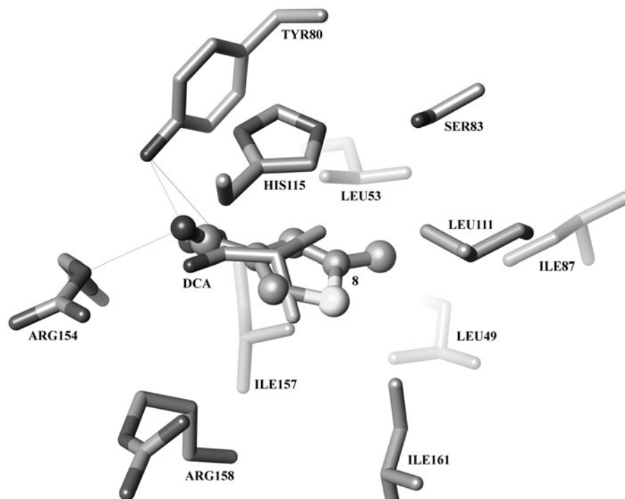
Figure 2. Predicted binding mode of compound 8 (balls and sticks) superimposed with the PDK2/DCA co-crystal structure 2BU8 (sticks).
